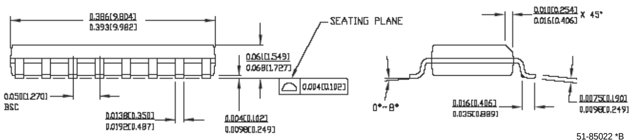
Figure 19. 16-Pin COL
